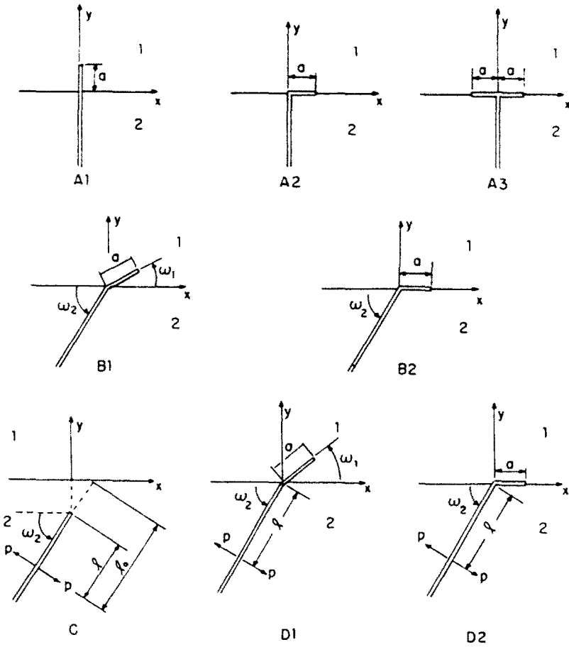
Fig. 1. Crack geometries.
